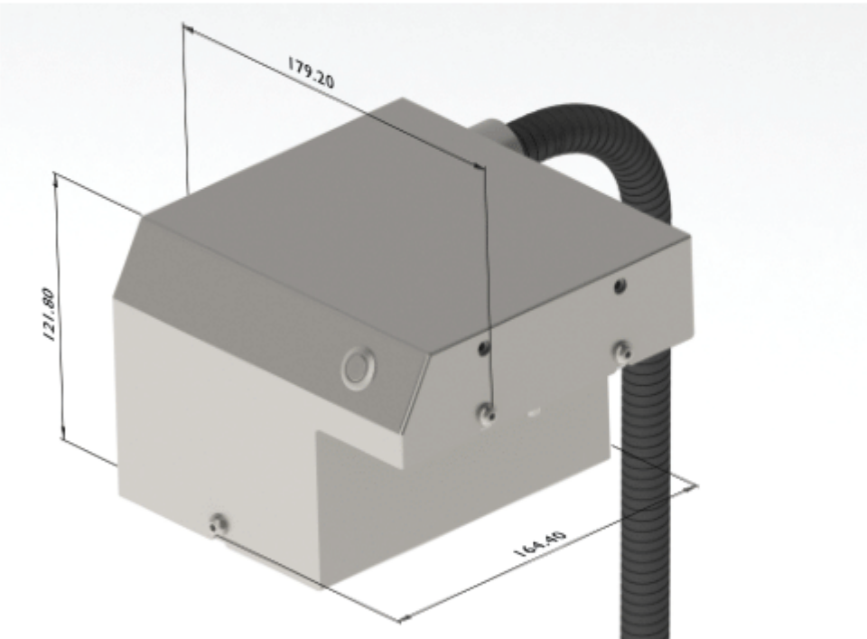
Remote printhead header tank
