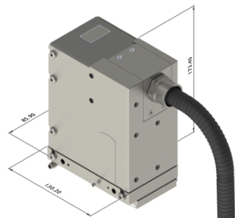
Remote printhead – vertical
