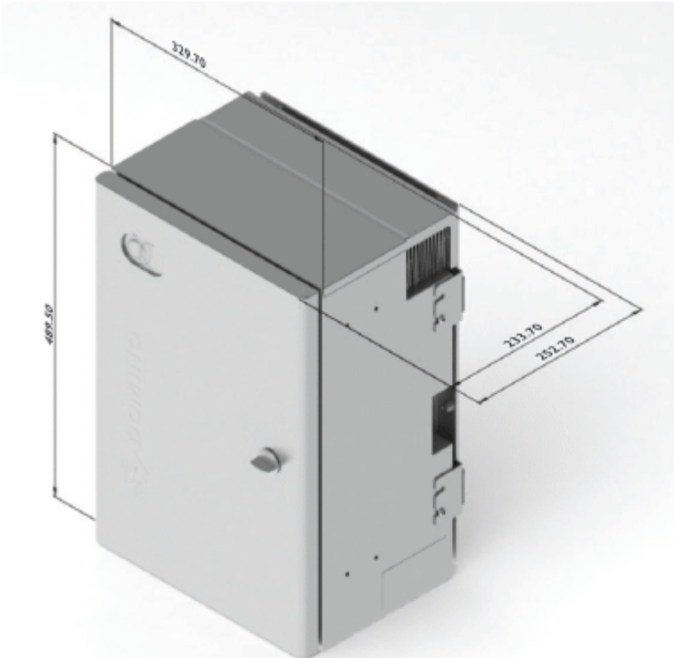
Base unit
