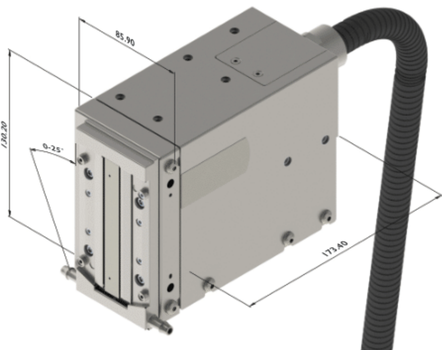
Remote printhead – horizontal
