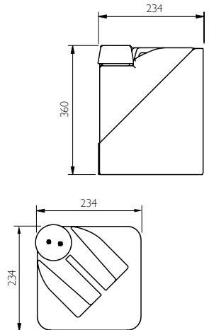
Flush holder
